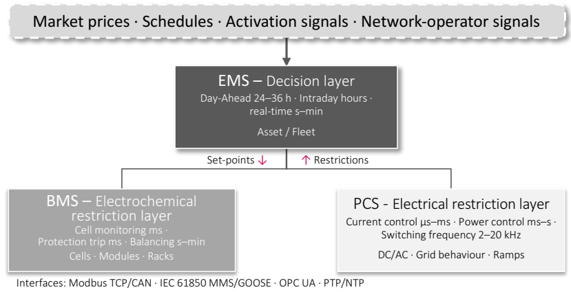
Figure 2. Asymmetric control architecture between BMS, EMS, and PCS. Restrictions ascend from the protection and conversion layers; set-points may only be passed downwards within these limits.
